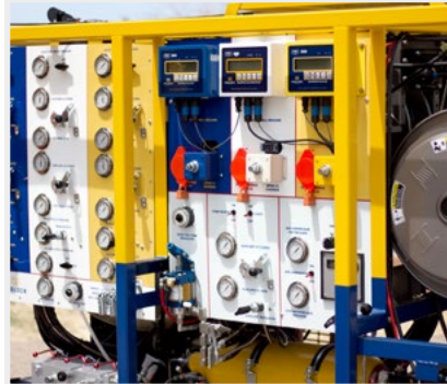
THE RIGLOCK MECHANISMS ARE CONTROLLED WITH A UNIQUELY DESIGNED HYDRAULIC CONTROL UNIT.
