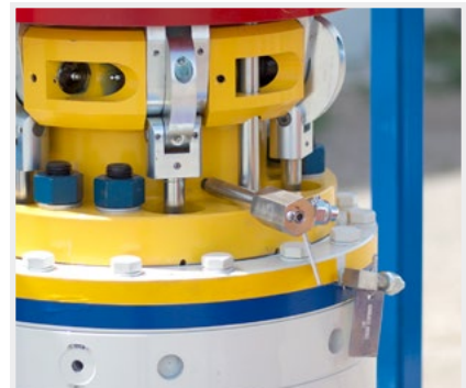
WITH AN INTEGRATED REGULATOR, THE RIGLOCK CAN TAKE THE PLACE OF YOUR QUICK TEST SUB.
